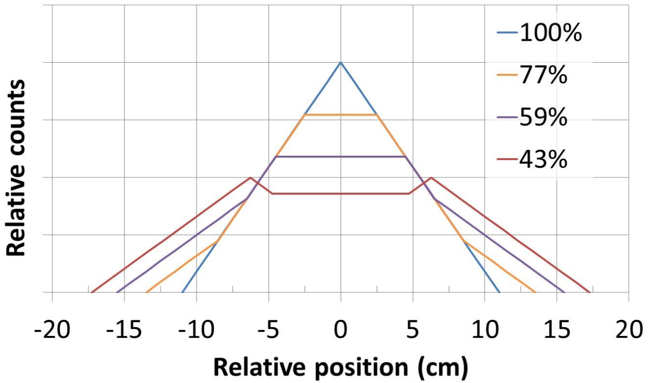
SUPPLEMENTAL FIGURE 3. Scan-length tailor-fitting in SS mode by adjusting amount of bed overlap.
