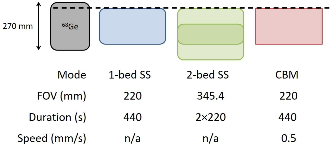
SUPPLEMENTAL FIGURE 1. Scan prescriptions for experimental verification of counting efficiencies in 3 acquisition modes.
