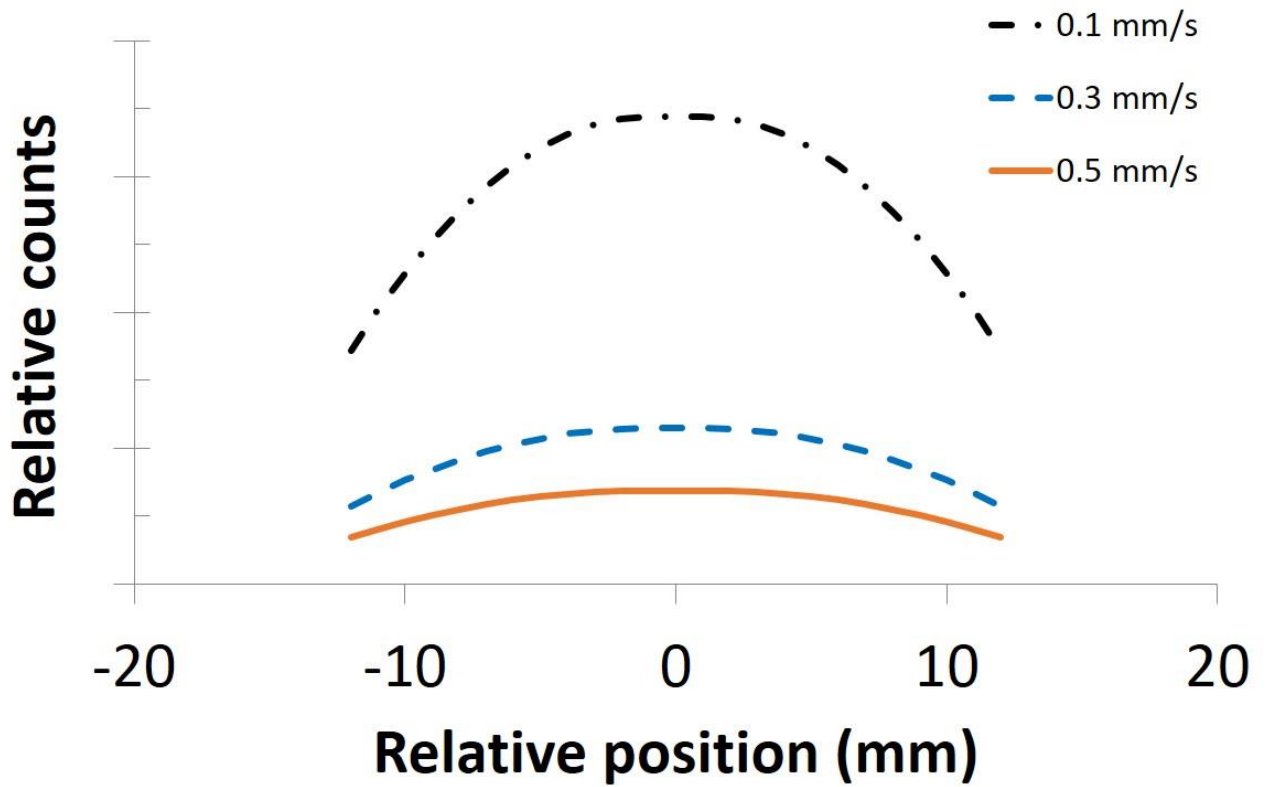
SUPPLEMENTAL FIGURE 2. CBM profiles variation in 1-aFOV (22-cm) scan as function of bed speed.
