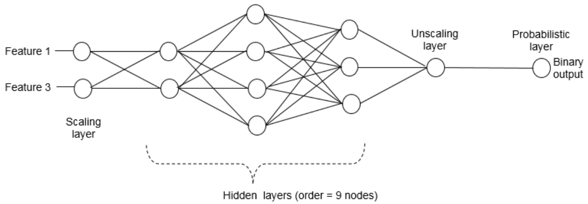
Supplemental figure 2: Final neural network architecture convolved from figure 7 with only 2 inputs, 3 hidden layers of 2, 4 and 3 nodes respectively, an unscaling layer and a single binary output.
