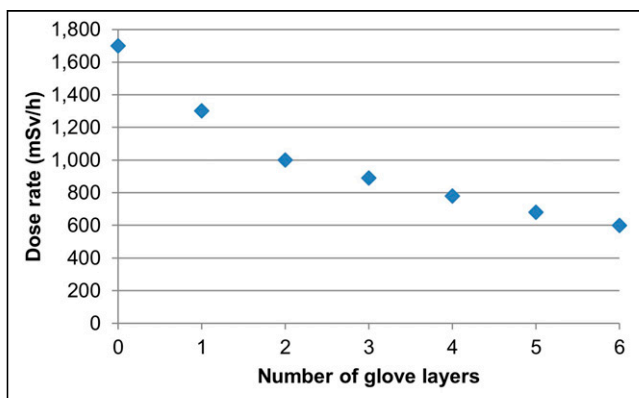
FIGURE 5. Dose rate (mSv/h) to 1 cm 2 of unbroken skin from 1-MBq (0.05 mL) droplet of 90 Y in relation to number of layers of 0.2-mm-thick surgical gloves covering unbroken skin.
