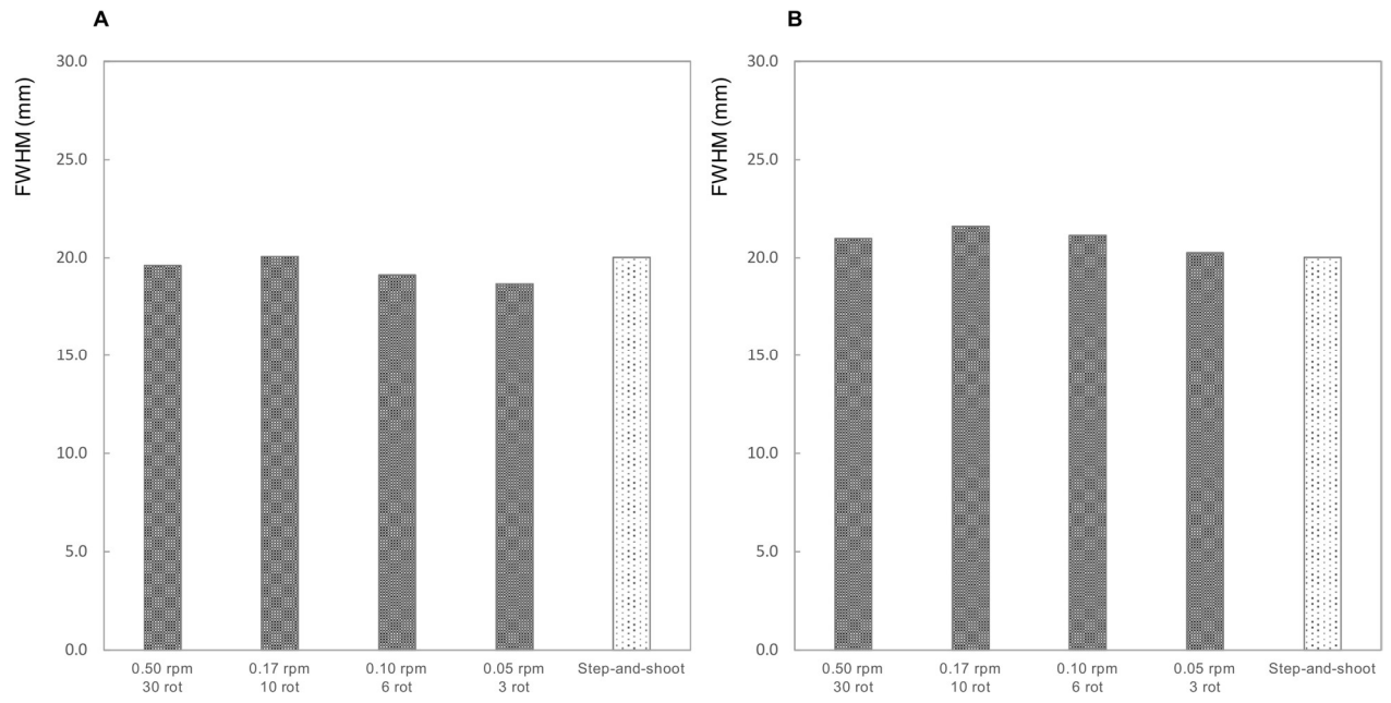
Fig. 3 Comparison of full width at half maximum (FWHM) results: (a) added projection data process, and (b) added reconstructed image process. The results were not clearly different among CRRA images acquired with each rotation parameter and the step-and-shoot mode.
