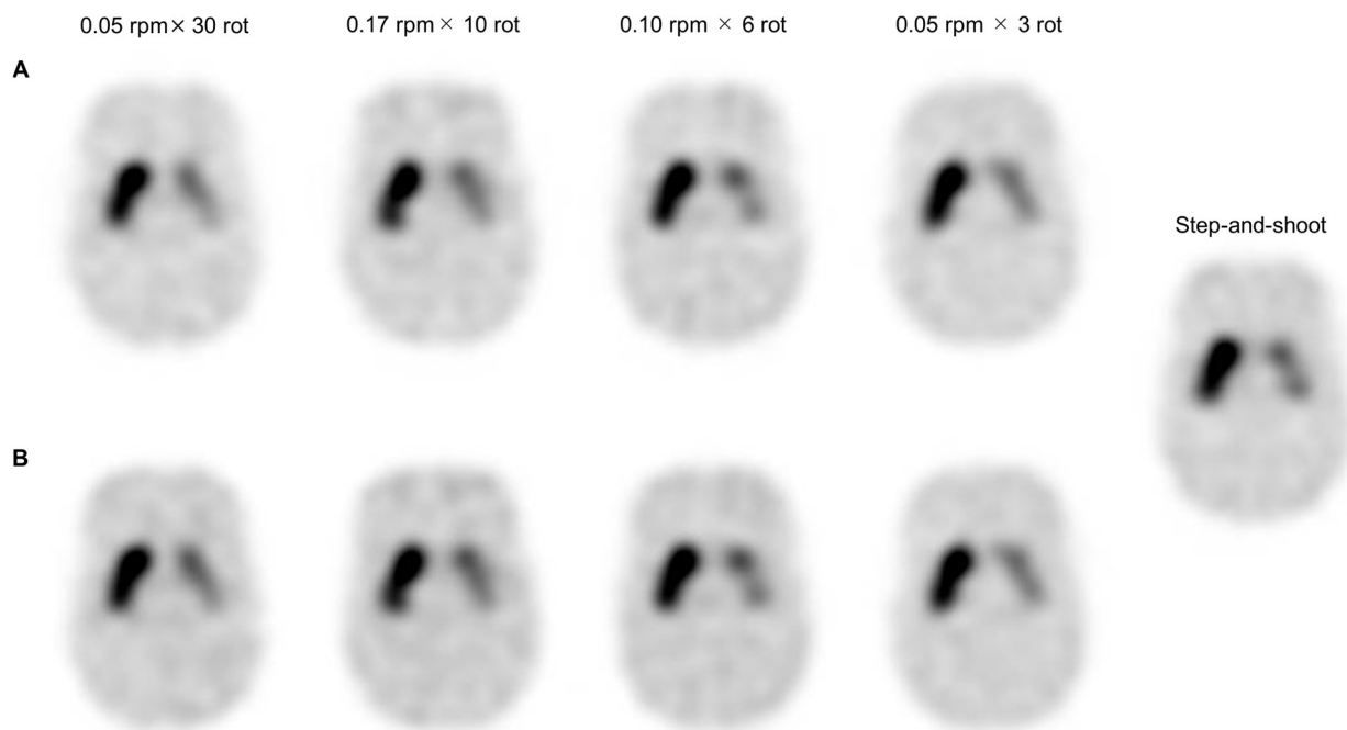
Fig. 6 Reconstructed images of the striatal phantom using CRRA and the step-and-shoot mode: (a) added projection data process and (b) added reconstructed image process. The uniformity of the background area decreased with a faster rotation speed.
