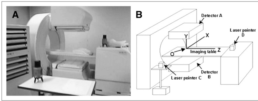
FIGURE 1. Appearance (A) and illustration (B) of pair of laser pointers aligned at right angles. Point O corresponds to center of rotation of detectors.
